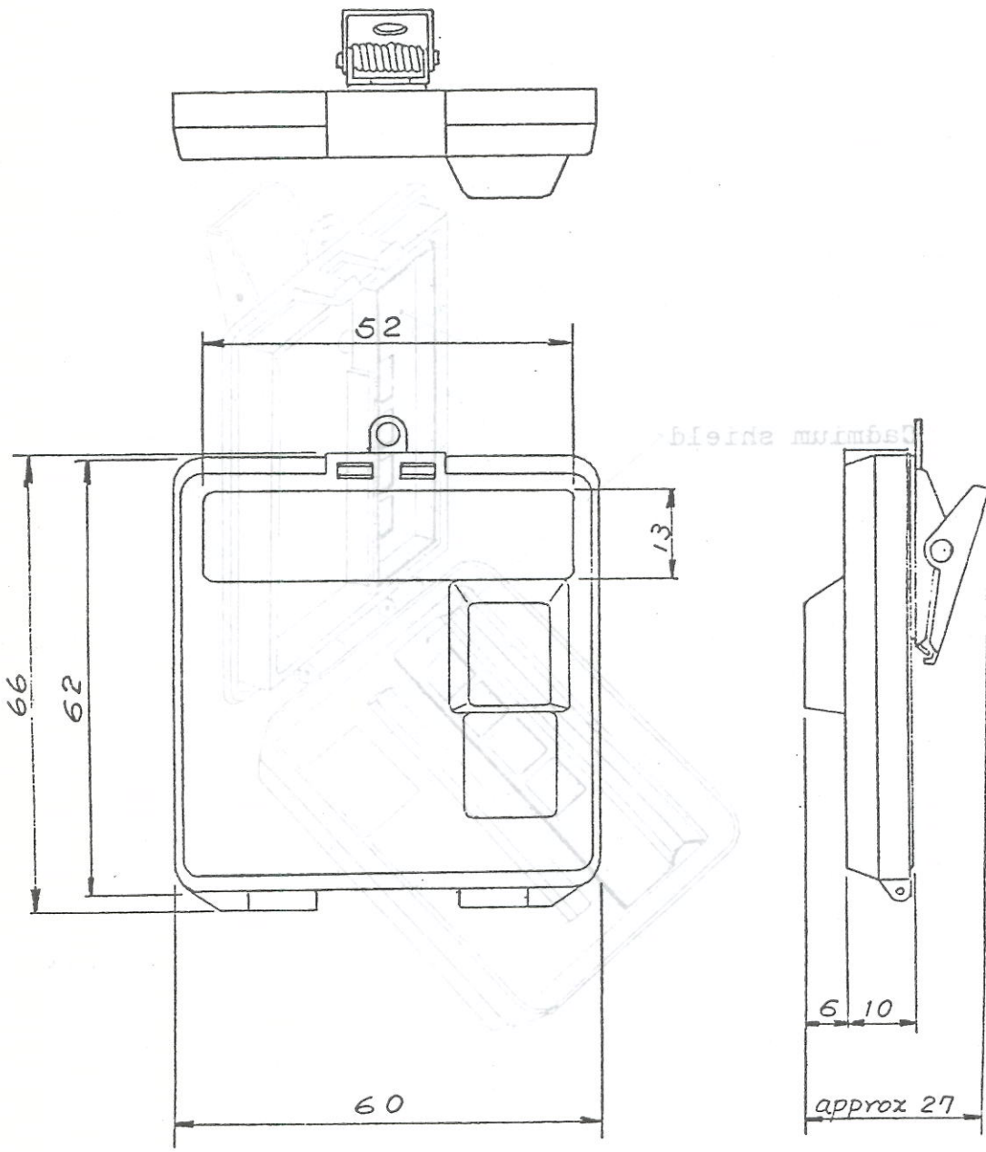
Fig.1 Structure of UD-887A-T.
