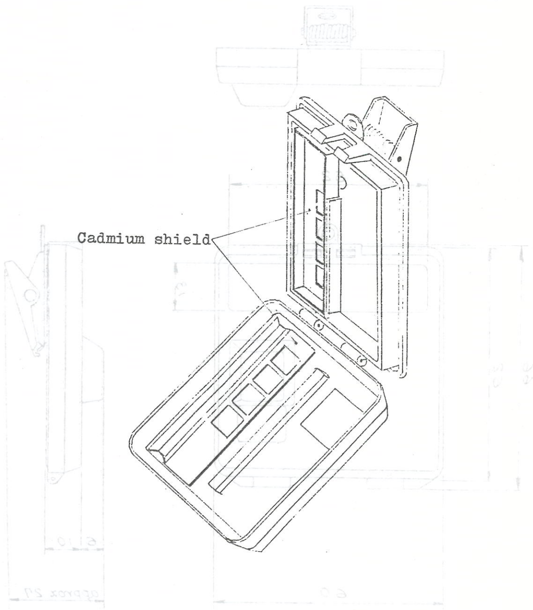
Fig.2 Inside of UD-885A-T
